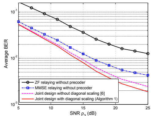
(b) BER versus \rho_2 with \rho_1 = 25\text{dB} .
