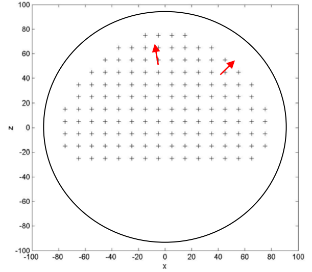
Fig. 1: Two dipoles inside the scalp sphere (x axis from back to front of the head). The scanning grid is shown with crosses.
