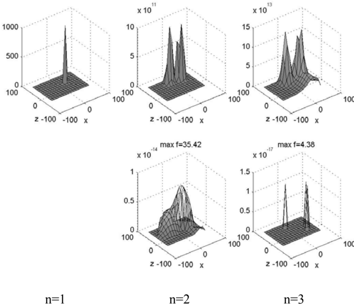
Fig. 2. Probabilistic maps obtained on the simulated dipoles (SNR of 20). Upper row: map 1. Lower row: map 2. Columns: number of sources in the scanning.
