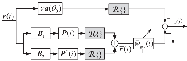
Fig. 3. Proposed WL reduced-rank scheme with the GSC structure.
