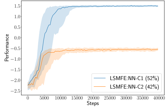
(b) Performance versus steps for investments example
