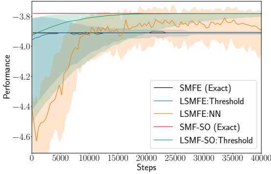
(a) Performance versus steps for malware spread example
