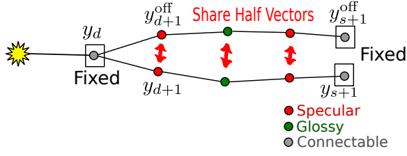
Figure 9: An example of a specular/glossy chain.
