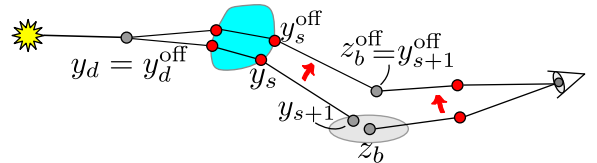
Figure 8: The case where y_s is unconnectable.
