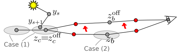
Figure 6: Gradient-domain vertex merging cases.
