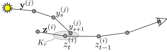
Figure 4: VCM paths.
