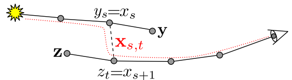
Figure 3: BDPT Paths.
