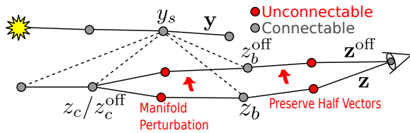
Figure 5: G-BDPT paths.
