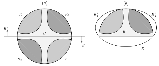
Fig. 1. The inductive step works by projecting K onto one less dimension. In (a) above, a projection on the horizontal axis would yield a distance of zero between the projected K_1 and K_2 . Once we bisect to obtain (b), we see that a projection onto the horizontal axis would not affect the minimum distance between K_1 and K_2 .
